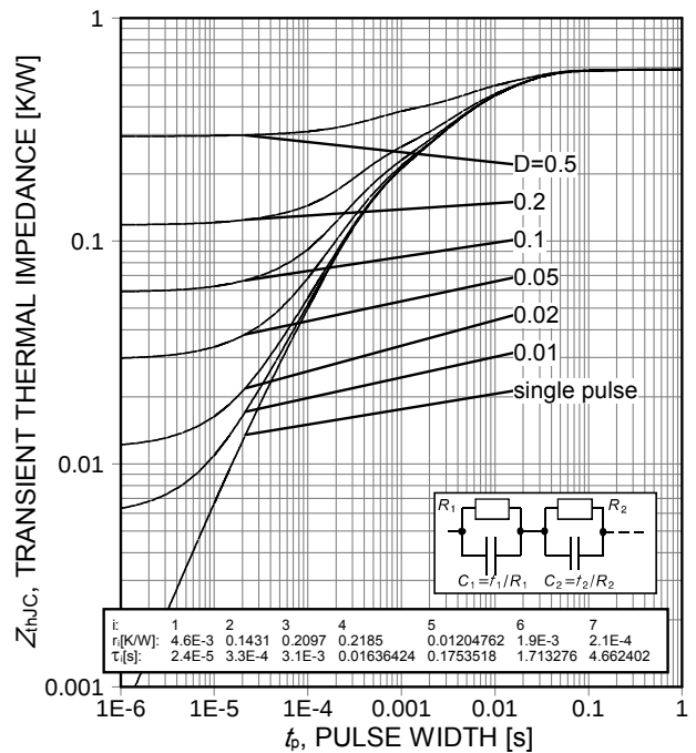
Figure 20. IGBT transient thermal impedance ( D=t_p/T )
