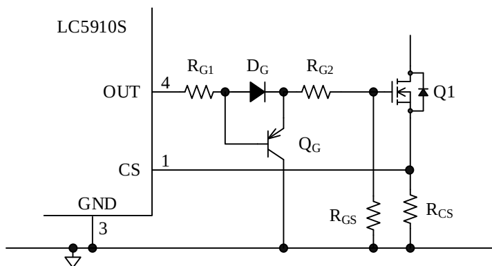
Figure 9-7. OUT Pin Peripheral Circuit (2)
