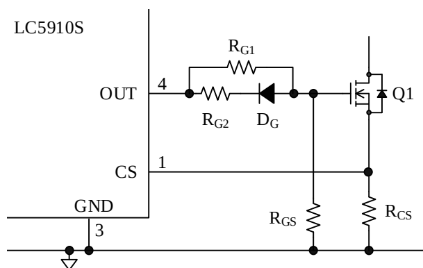
Figure 9-6. OUT Pin Peripheral Circuit (1)
