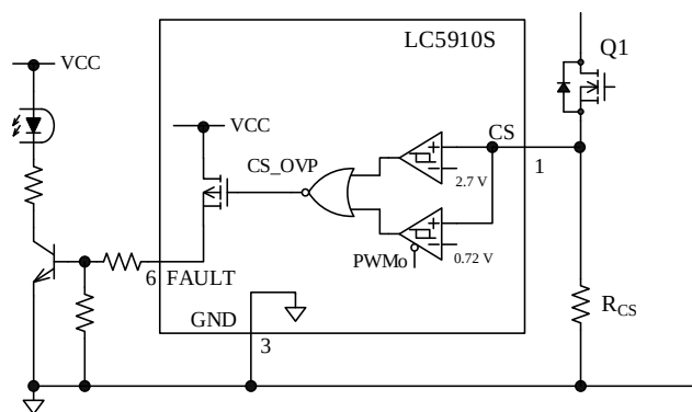
Figure 9-9. FAULT Pin Peripheral Circuit
