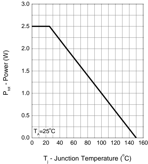
Power Dissipation
