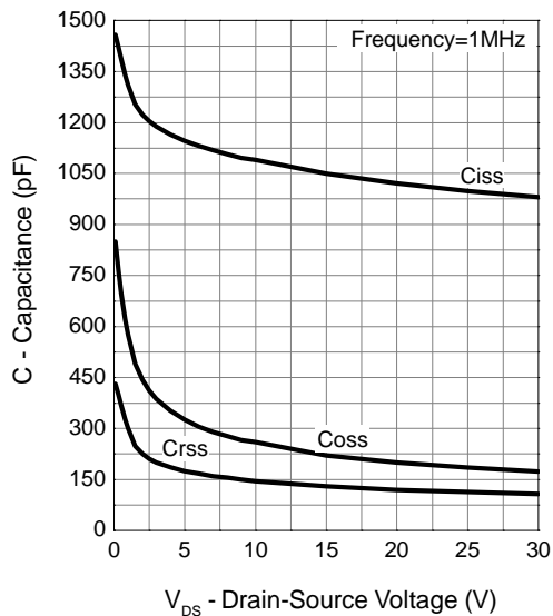
Capacitance
