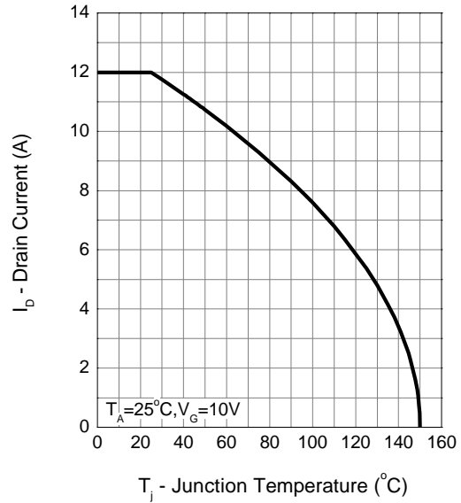
Drain Current
