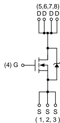
N-Channel MOSFET
