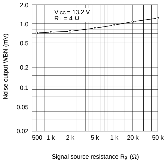
Figure 6 Noise Output vs. Signal Source Resistance
