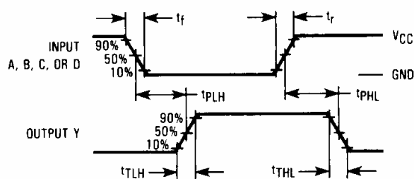
Figure 1. Switching Waveforms
