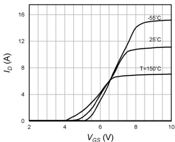
Fig.5 Transfer Characteristics
