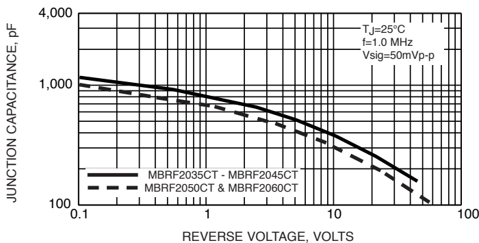
FIG. 5 - TYPICAL JUNCTION CAPACITANCE PER LEG
