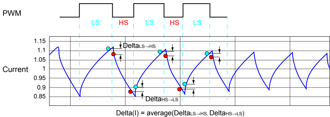
Figure 19. HS/LS current compare example
