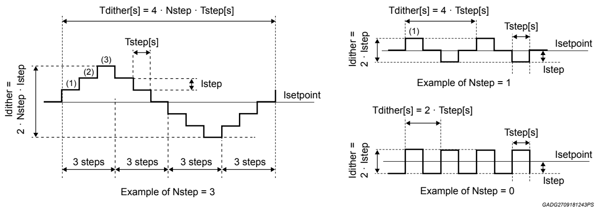
Figure 13. Dither waveforms definitions
