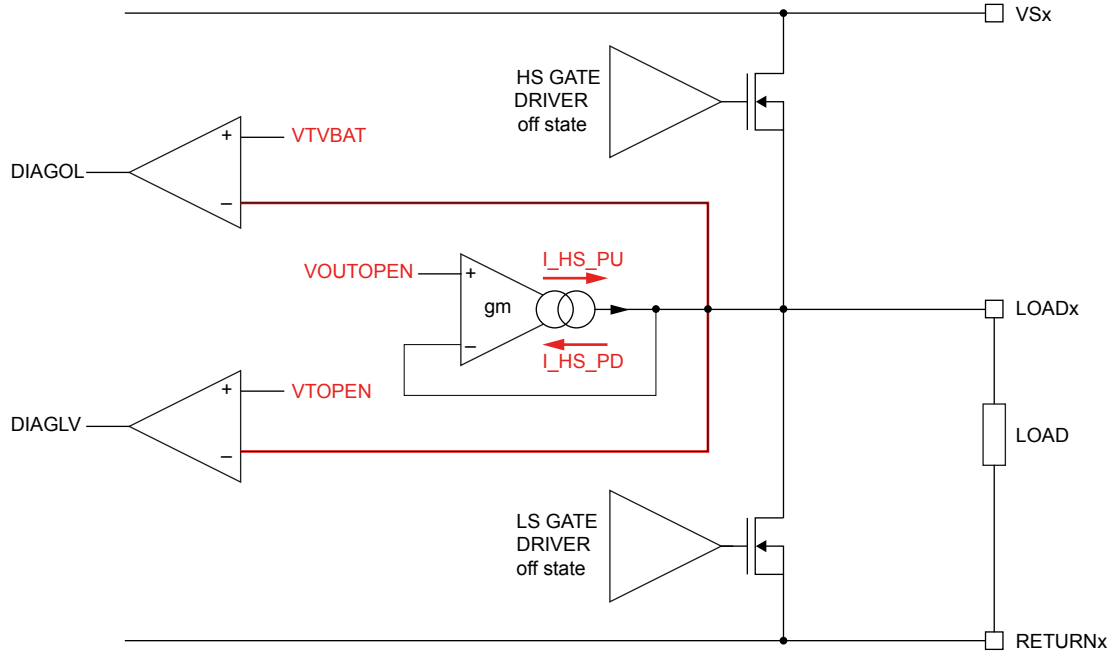
Figure 16. High side configuration diagnostic
