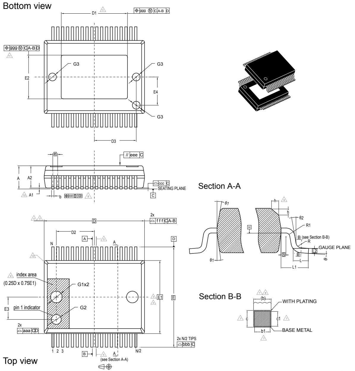
Figure 31. PowerSSO-36 (exposed pad down) package outline
