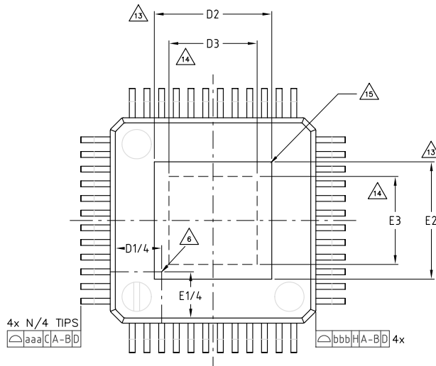
Figure 28. TQFP48 (7x7x1 mm exp. pad down 5.0x5.0) package outline
