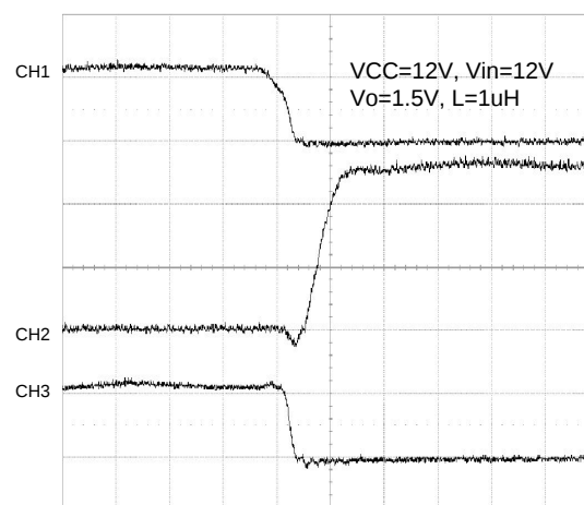
UGATE Falling
