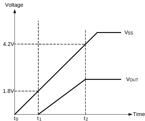
Figure 1. Soft-Start Internal
