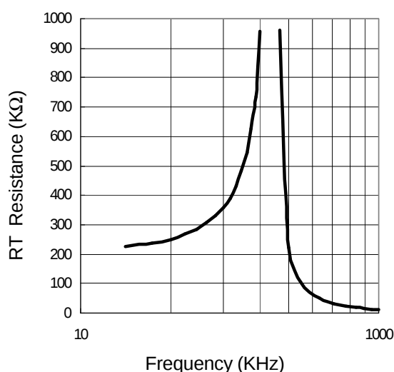
Figure2. Oscillator Frequency vs. RT Resistance
