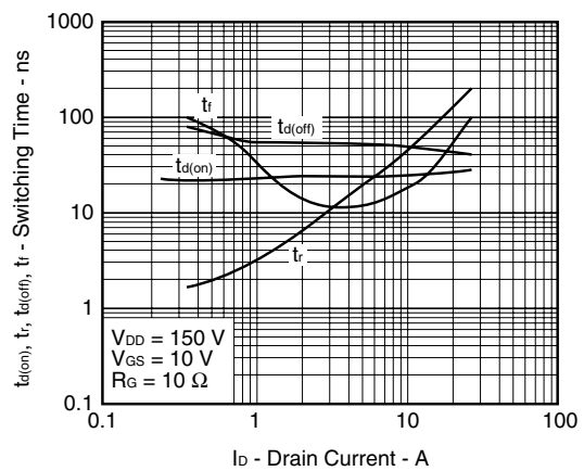
SWITCHING CHARACTERISTICS
