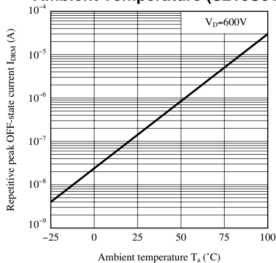
Fig.8-b Repetitive Peak OFF-state Current vs. Ambient Temperature (S216S01)
