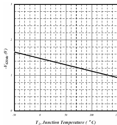
Fig 12. Gate Threshold Voltage v.s. Junction Temperature
